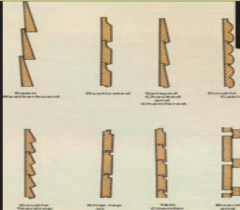
SHIPLAP PROFILES
